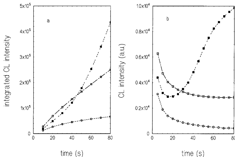
Fig. 1. Co 2+ (■) and Mg 2+ (□) effects on time variation of the chemiluminescence. Reference system: LH 2 (2 μM)–H 2 O 2 (25 μM) in Tris–HCl buffer, pH 8.32 (○).
